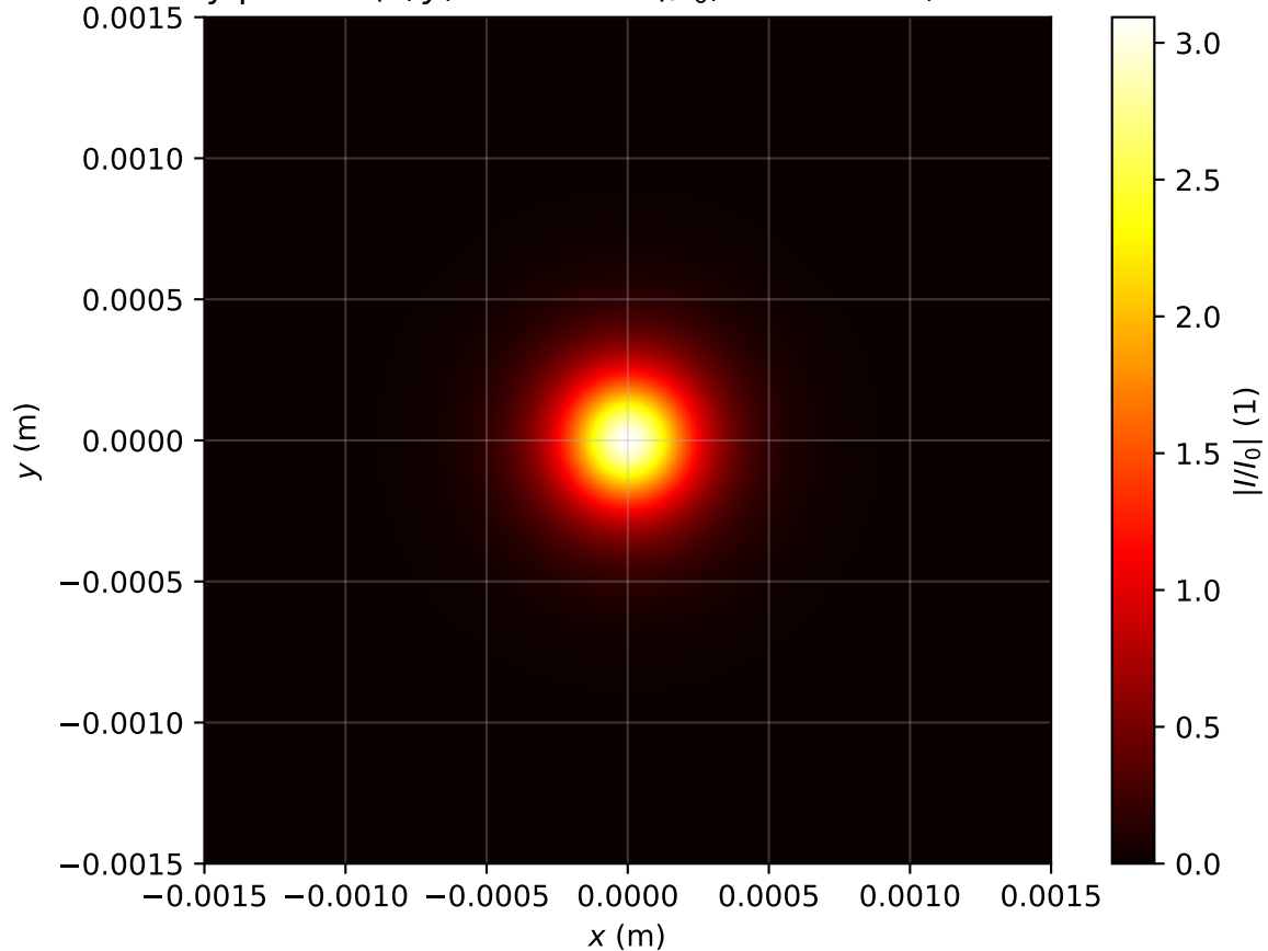
Intensity profile I(x, y, z = 3.662m)/I_0 , Pin=1.0Pcr, artificial time
